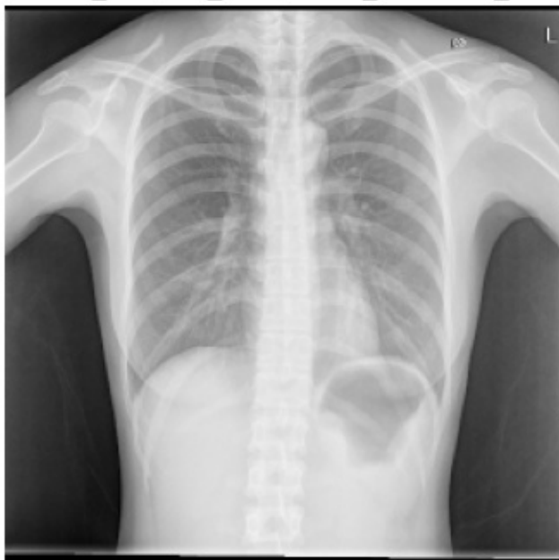
16base_5depth_0.1spatial_32batch_0fold
