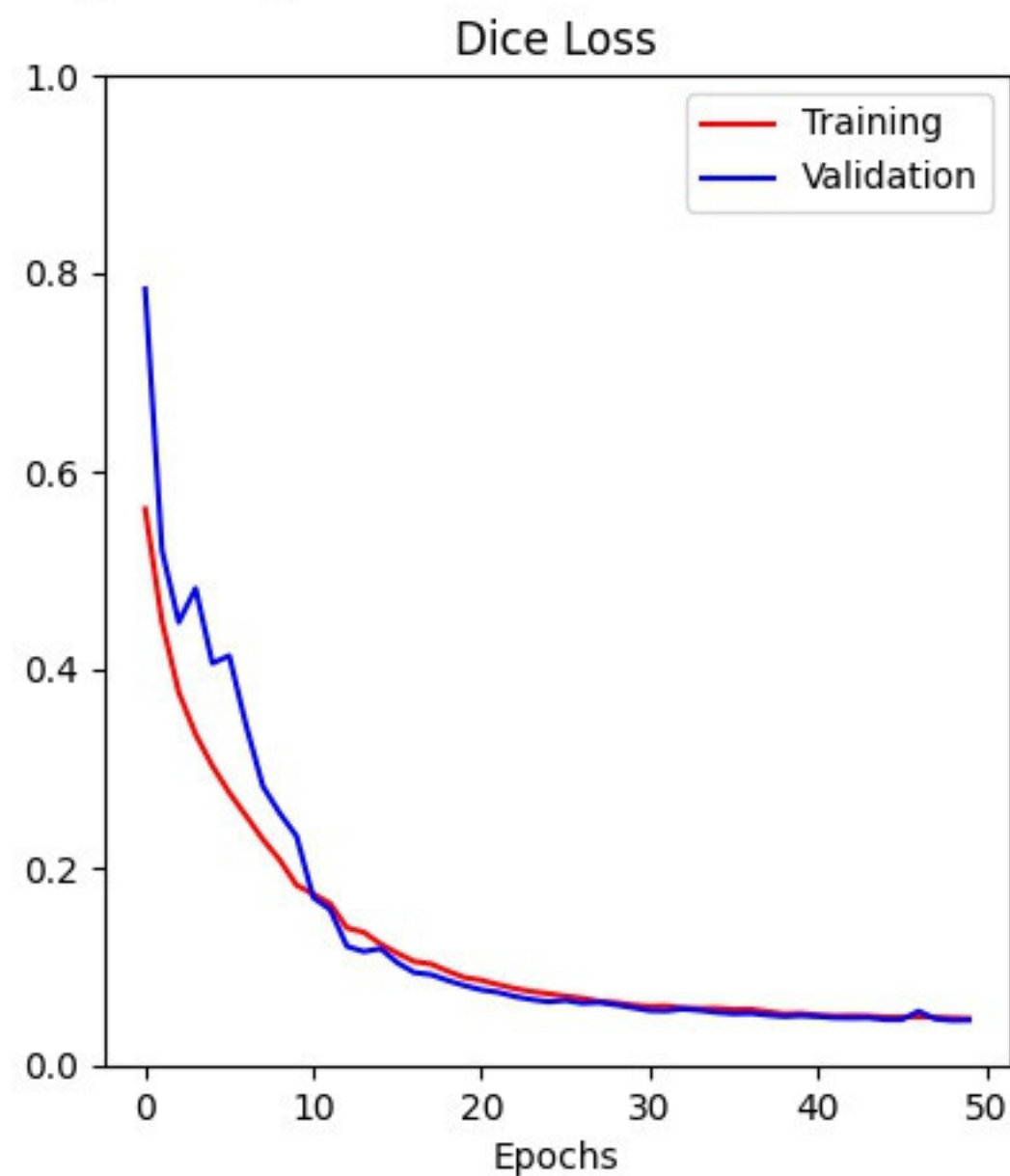
8base_6depth_0.1spatial_32batch_0fold
