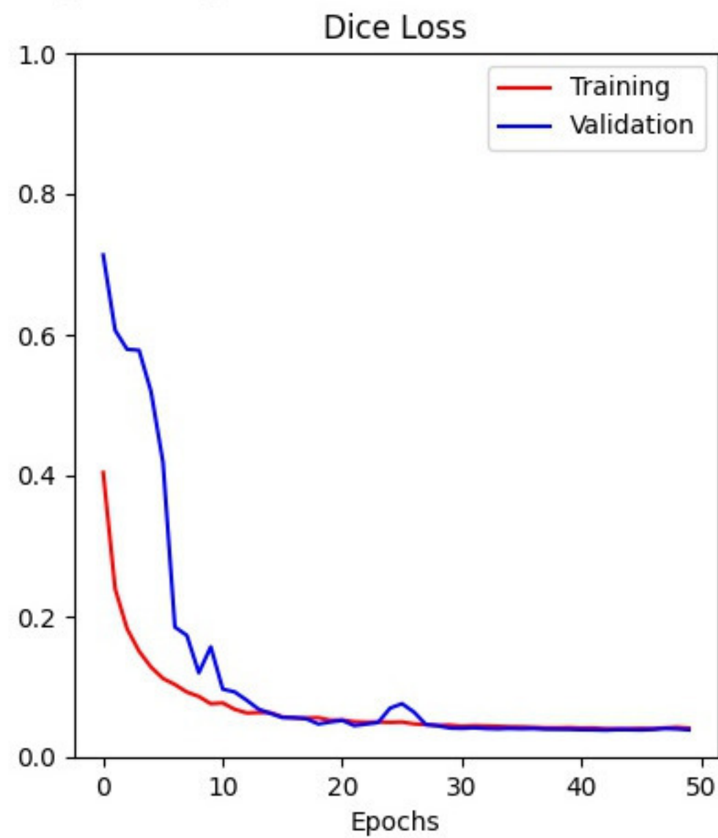
16base_5depth_0.1spatial_32batch_0fold
