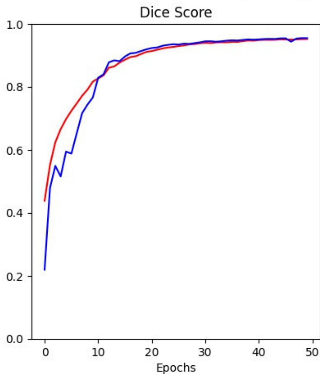
8base_6depth_0.1spatial_32batch_0fold
