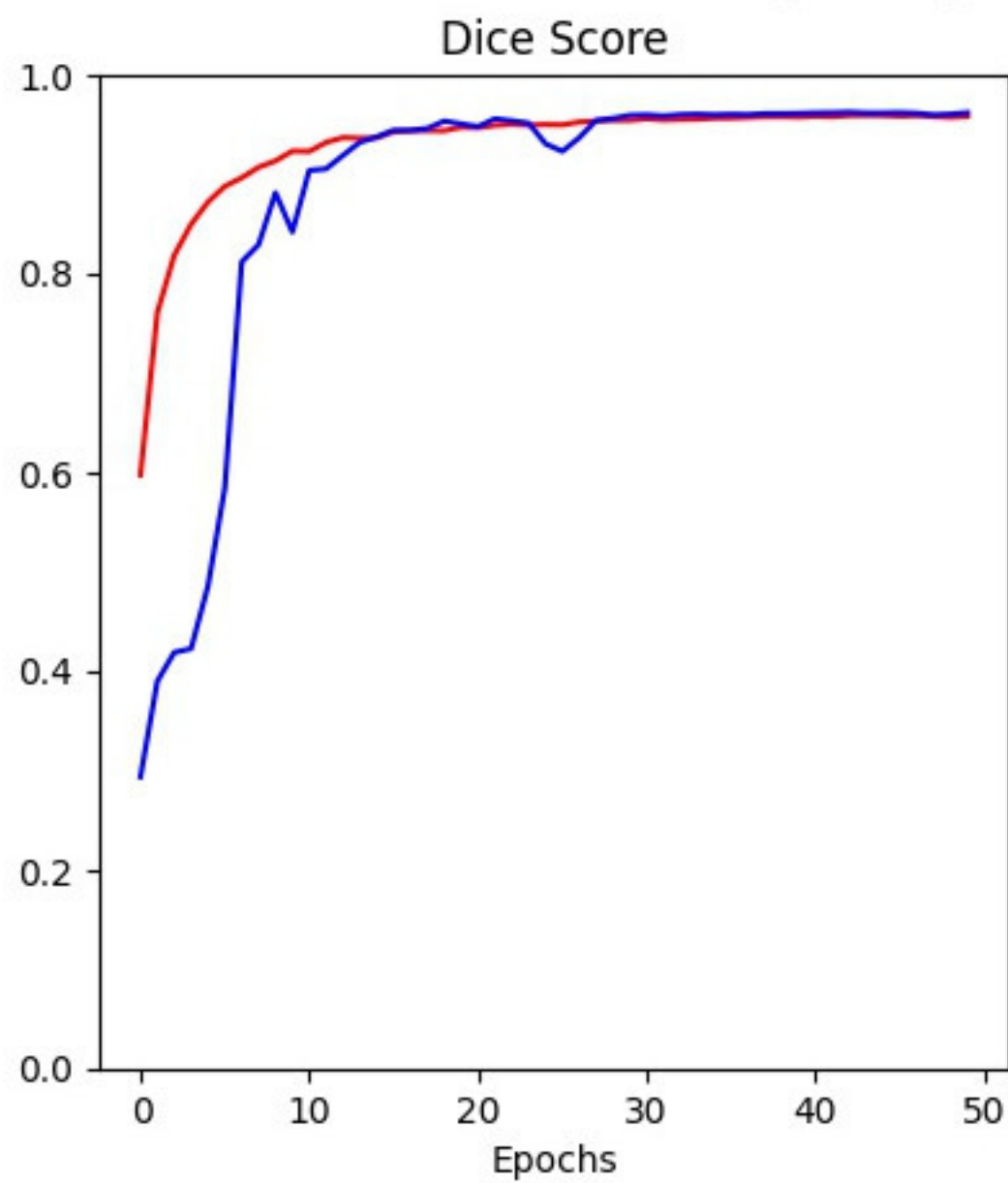
16base_5depth_0.1spatial_32batch_0fold
