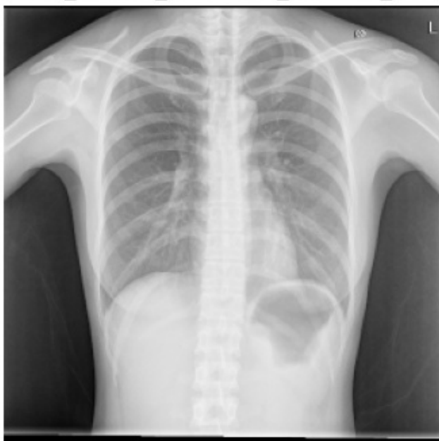
16base_5depth_0.1spatial_32batch_0fold
